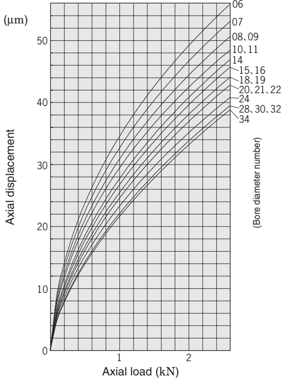
(11) HAR900 series (contact angle : 30°)
