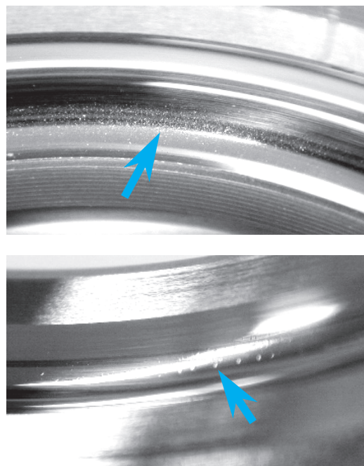
Fig. 1.2 Example of biting flaws formed in raceway because of entry of foreign particle
