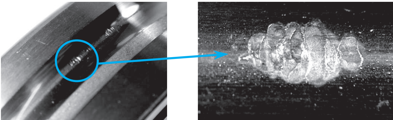
Fig. 1. 4 Example of flaking
